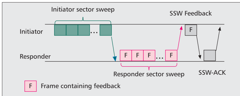
Figure 5. Sector-level sweep.
