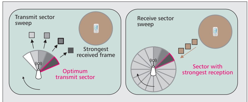
Figure 6. Transmit and receive sector training.
